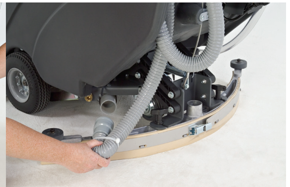
For a full-functioning extractor, move the hose to the vacuum shoe inlet and raise the squeegee.
